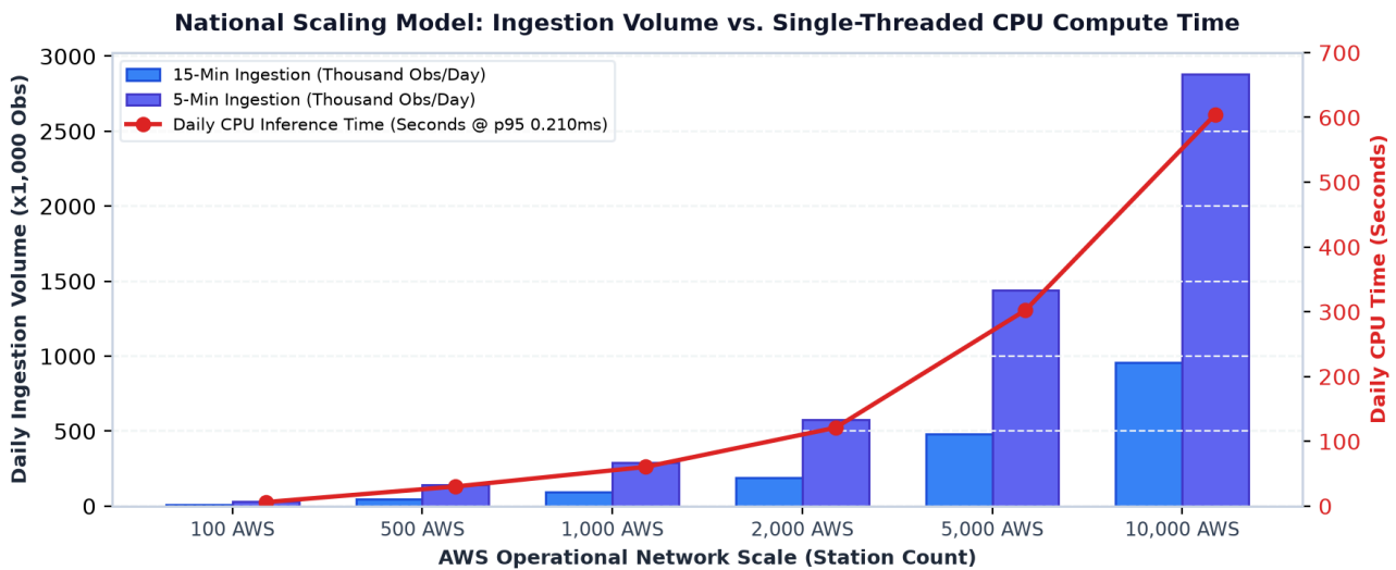
Figure 4: National Scaling Compute Workload. Daily CPU compute time required across scaling station counts (100 to 10,000 AWS) at 5-minute sampling cadences, executing high-efficiency vectorized processing.
